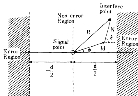
그림 7 Phasor diagram of received signal point corrupted by interfere point and impulsive noise.
