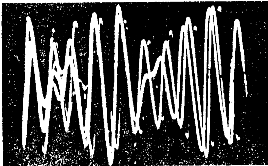
그림 3 Distortion of QAM wave in co-channel interference (time base 0.2mS/cm).
