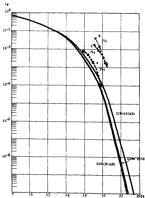
그림 12 The error probability in the environment of cochannel interference ( A=1, \Gamma'=100, CIR=10, 20, 30 (dB)).
