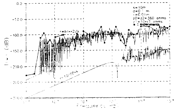
(b) 송진단이 개방되었을 경우 (b) the case with the sending end open-circuited
