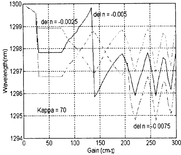
그림 9. \Delta n_2 의 변화에 따른 tuning trend( \lambda/4 phase shifted 3전극 DFB-LD) Fig. 9. The tuning trend about a change of \Delta n_2 (The three section DFB-LD with a \lambda/4 phase shift)
