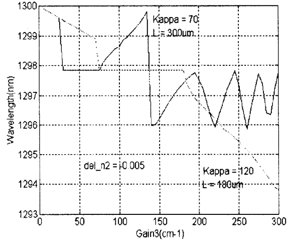
그림 10. Coupling 상수에 따른 tuning trend( \lambda/4 phase shifted 3전극 DFB-LD) Fig. 10. The tuning trend about a coupling coefficient(The three section DFB-LD with a \lambda/4 phase shift)
