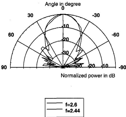
Fig. 5 Radiation pattern of a horn antenna at 2.4 and 2.6 GHz
