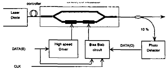
Fig. 2 Experimental set-up for the demonstration.
