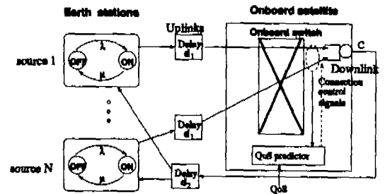
Fig. 1 Congestion prediction and control architecture for broadband satellite communication.
