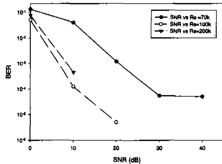
Fig. 4 BER performance with different symbol rates
