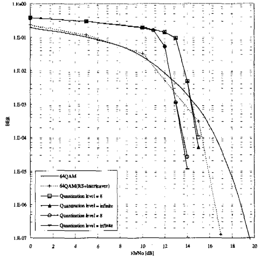
(a) 64-QAM
