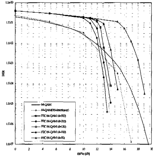
(a) 64-QAM
