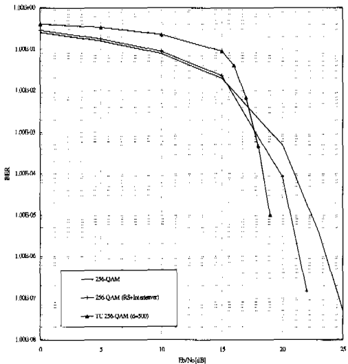
(b) 256-QAM
