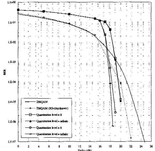
(b) 256-QAM
