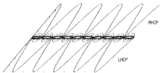
Fig. 2 Subchannel spectrum of the XCP-OFDM
