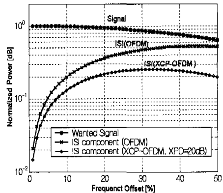
Fig. 7 The Power of the Signal and ICI
