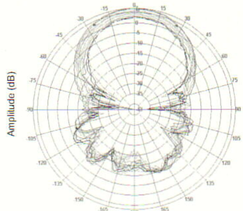
(a) E-평면
