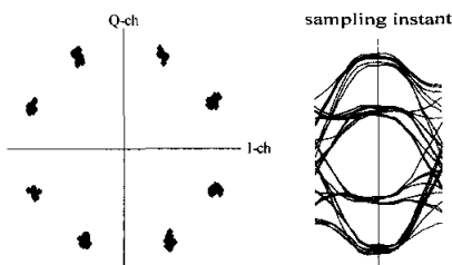
(a) 8SQAM(A=B=0.6, IBO=5dB)
