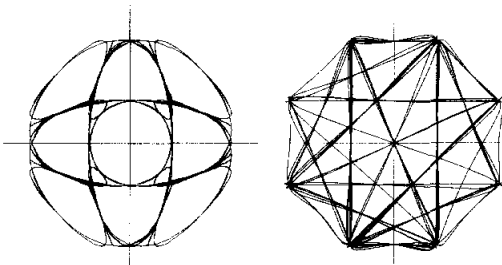
(a) 8SQAM(A=0.7) (b)8PSK (α=1.0)
