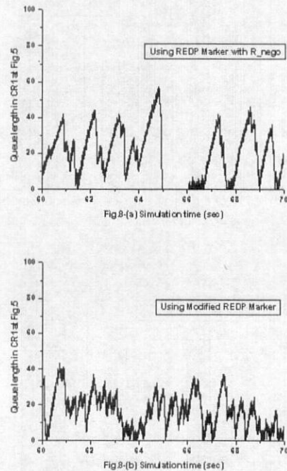
Fig.8. Comparison of queue length variations
