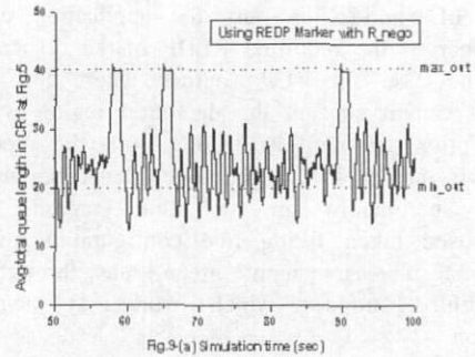
Fig.9(a) Simulation time (sec)
