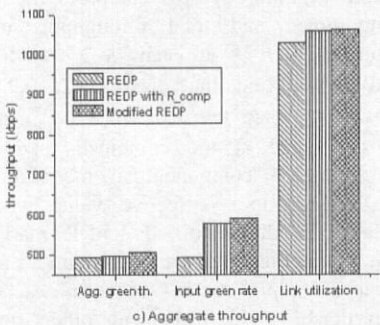
Fig.11. Fairness and aggregate throughput at Fig.10.
