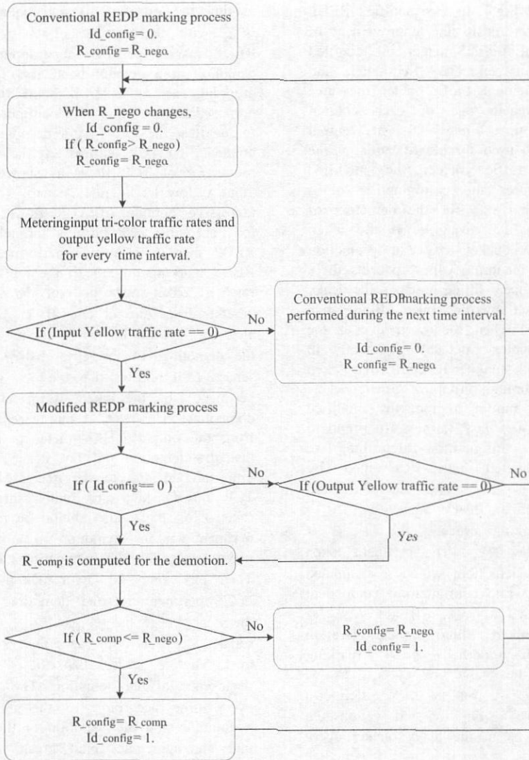
Fig.4. Token filling rate configuration algorithm.
