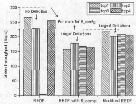
(a) Green throughput
