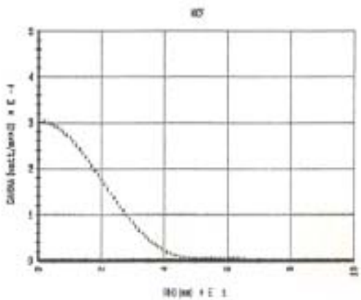
Fig. 2 The obtained mutual coherence function, \Gamma(\rho)
