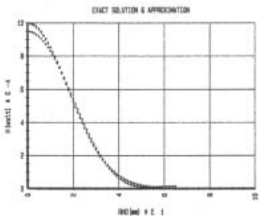
Fig. 3 the exact solution and approximation of H_T(\rho)
