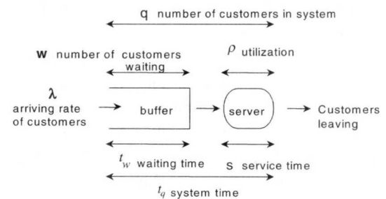
Fig. 2. Queueing system.
