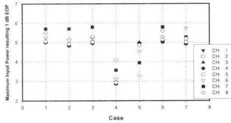
(b) D_{av} = 0.8 ps/nm/km
