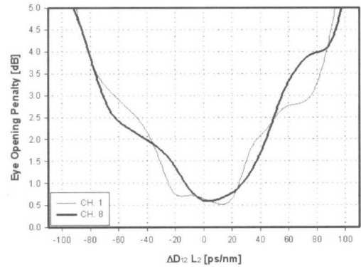
(b) D_{11} = 0.8 ps/nm/km ; P_s = 4 dBm
