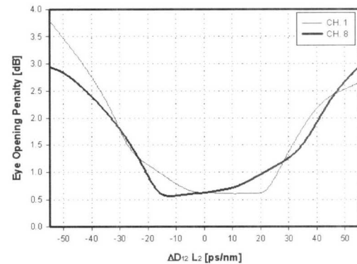
(c) P_s = 5 dBm
