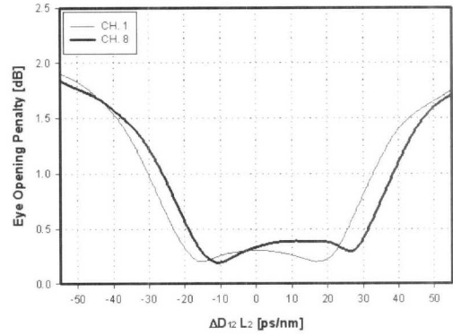
(a) P_s = 0 dBm
