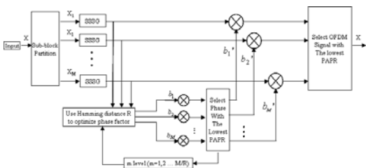
Fig. 4. Structure of Hybrid algorithm
