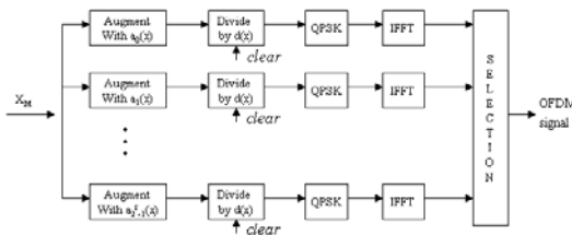
Fig. 5. Signal selection set generation (SSSG)
