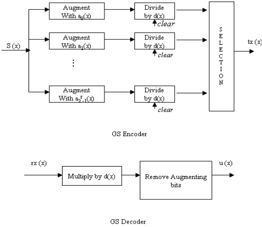
Fig. 2. Guided scrambling implementation
