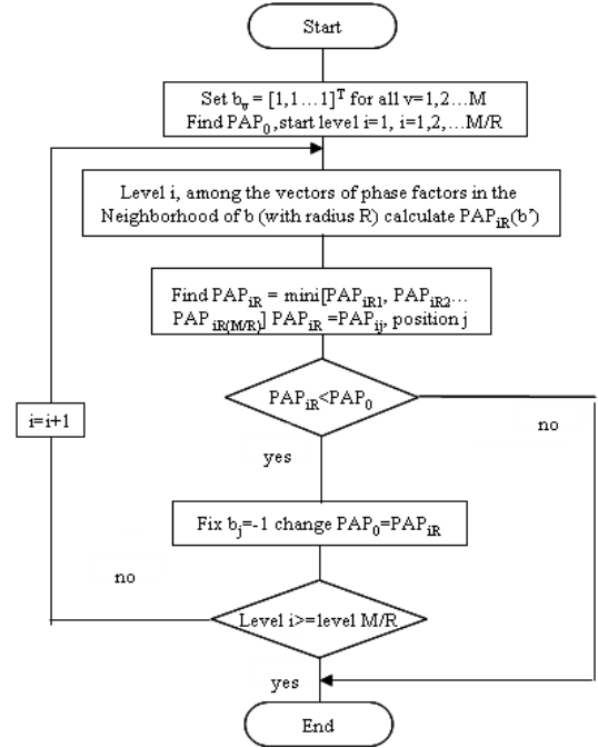
Fig. 3. The proposed weighting factor optimization method
