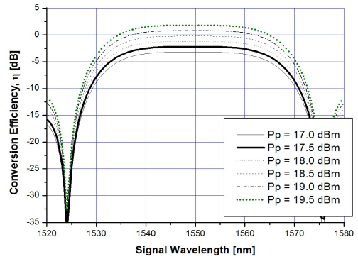
Fig. 3. The calculated value of conversion efficiency
