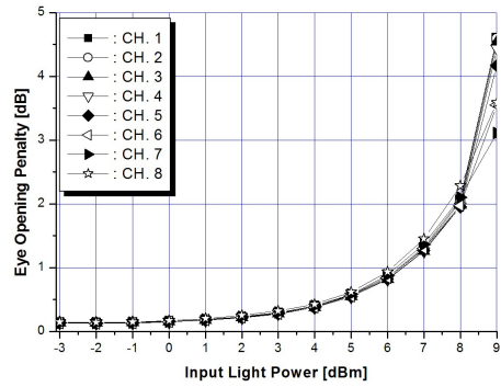
(b) D=0.4 ps/nm/km ; P_p=18.42 dBm
