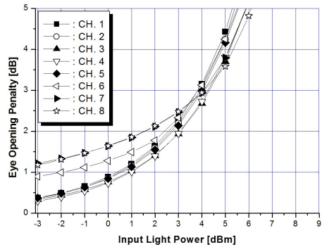
(h) D=1.6 ps/nm/km ; P_p=19.05 dBm
