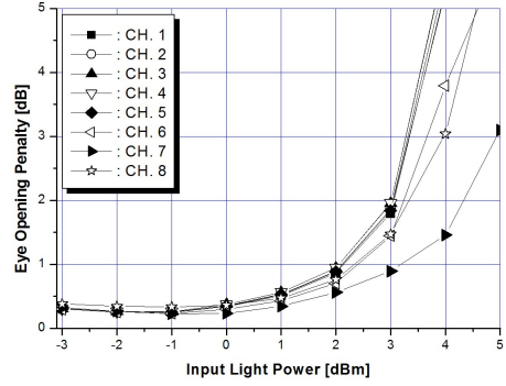
(b) D=0.4 ps/nm/km ; P_p=18.54 dBm
