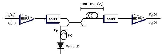
Fig. 2. Configuration of OPC using HNL-DSF
