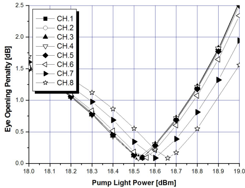
(a) l=40 km ; D=0.1 ps/nm/km ; NRZ
