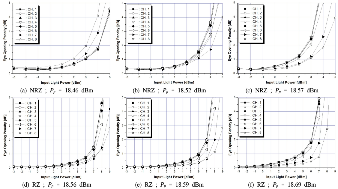
Fig. 6. EOP of overall NRZ and RZ channels as a function of the P_s at the P_p presented in Table 3 in the case of l=50 km and D=0.4 ps/nm/km.
