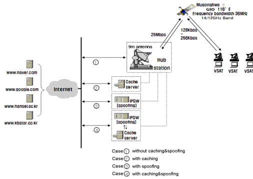
Fig. 3. Satellite test network configuration for improved protocol
