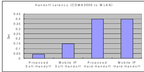
(b) cdma2000 to WLAN
