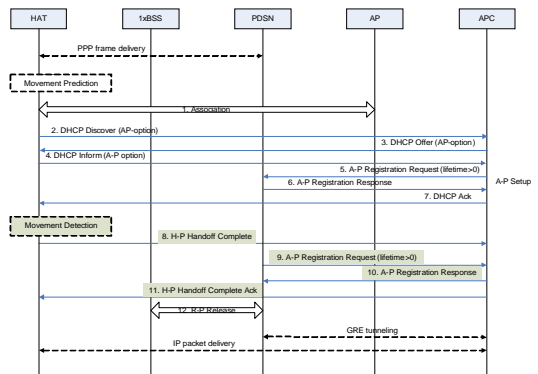
(a) cdma2000 to WLAN
