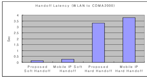
(a). WLAN to cdma2000
