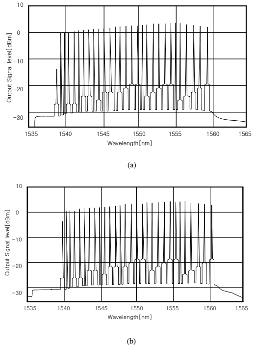
Figure 6. Signal spectra (a) without NPOT (b) with NPOT
