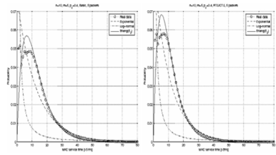
Fig. 5 PDFs : B(z) (Basic vs. RTS/CTS, p_c=0.4 )
