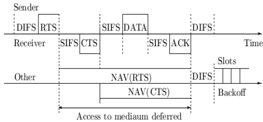
Fig. 2 RTS/CTS access mechanism
