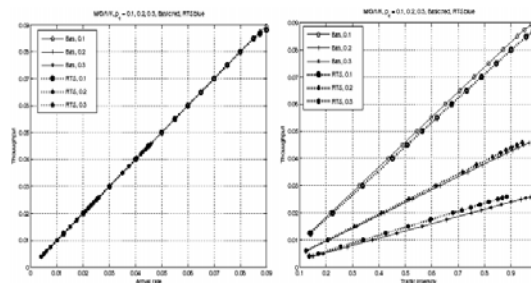
Fig. 8 System throughput w.r.t. \lambda and \rho
