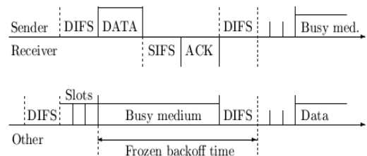
Fig. 1 Basic access mechanism
