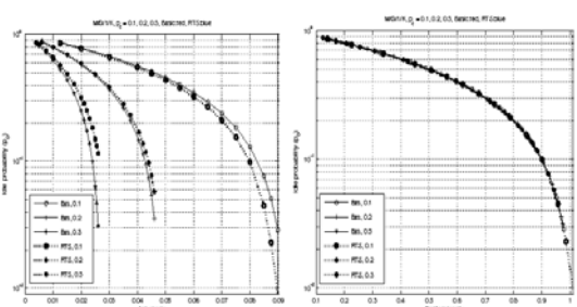
Fig. 9 Idle probability( p_0 ) w.r.t. \lambda and \rho
