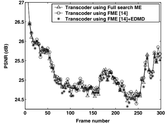
Fig 7. PSNR’s resulted from transcoder (358 kbps → 148kbps, 15Hz →15Hz) for a CIF ‘Mobile & Calendar’ sequence.
