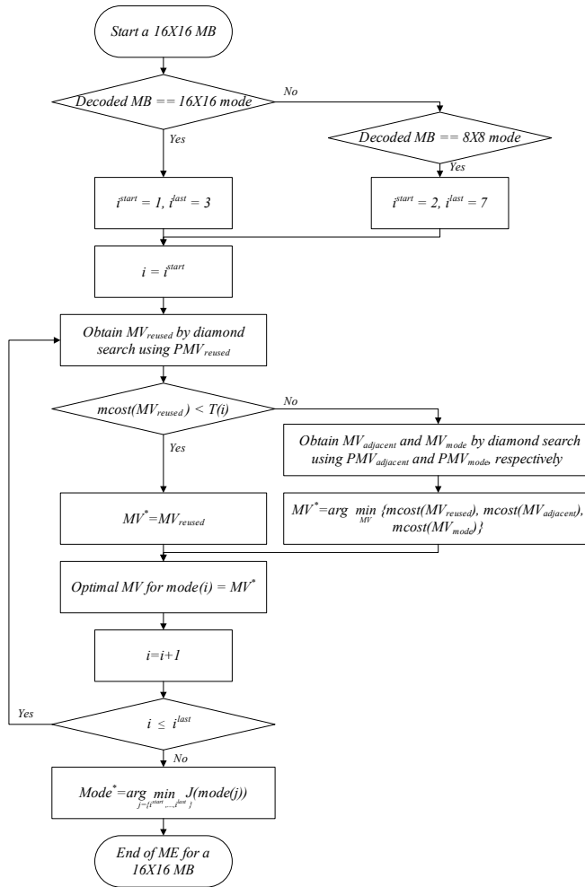
Fig. 3. The proposed ME procedure for a macroblock.
