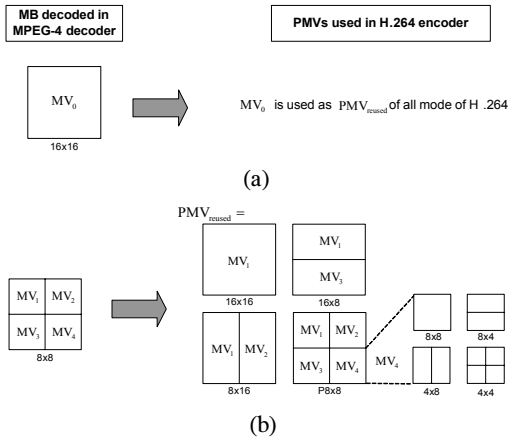
Fig. 1. PMV_{reused} for H.264 encoder is set to one of MVs decoded in MPEG 4 decoder part. : (a) When decoded MB is 16x16 mode, PMV_{reused} 's of all modes are set to the decoded MV (i.e., MV_0 ), (b) When decoded MB is 8x8 mode, PMV_{reused} of each mode is selected from one of the decoded 4 MVs (i.e., MV_1 , MV_2 , MV_3 , and MV_4 ).
