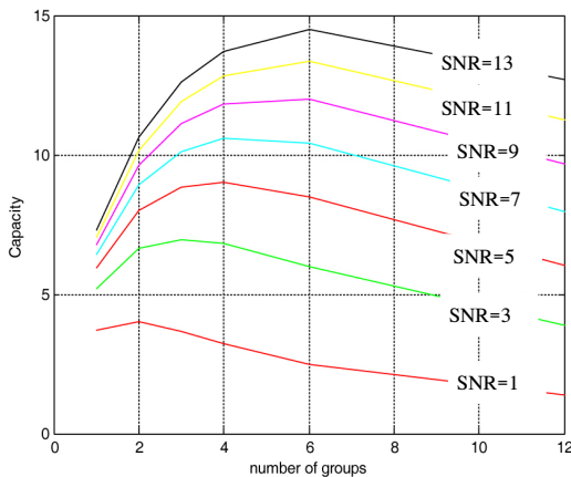
Fig. 5. Capacity according to the number of groups with different SNR in separate channel case.
