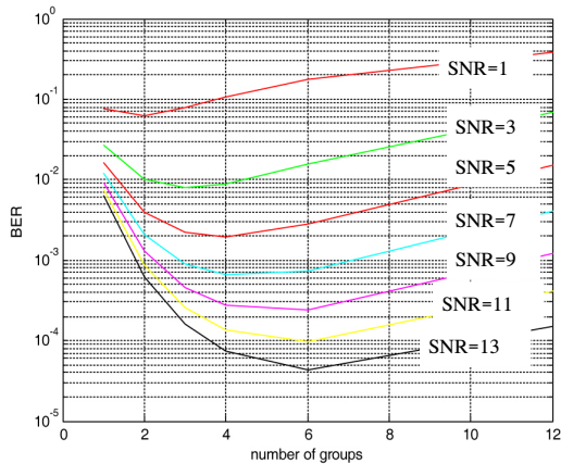
Fig. 4. BER according to the number of groups with different SNR.
