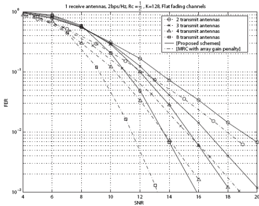
Fig. 4. Frame-error-rate performance comparison for various transmit and one receive antennas
