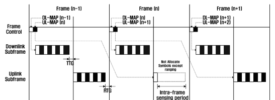
(a) TDD
