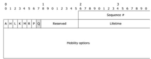
(a) Proxy Binding Query (PBQ)
