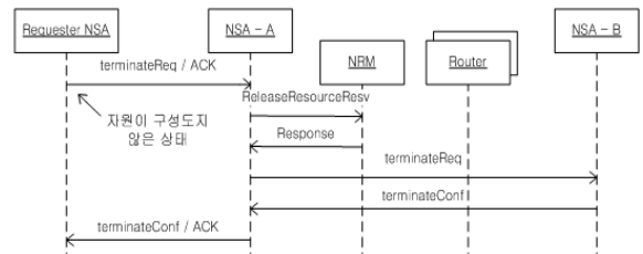
Fig. 6. NSI Termination message flow (Nonprovisioned Connection)
