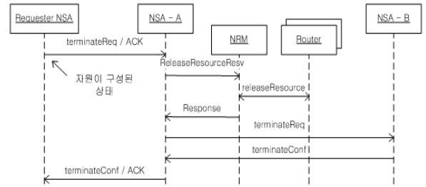
Fig. 5. NSI Termination message flow (Provisioned Connection)
