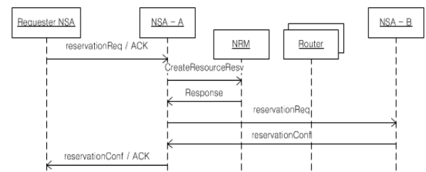
Fig. 2. NSI Reservation message flow
