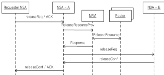
Fig. 4. NSI Release message flow
