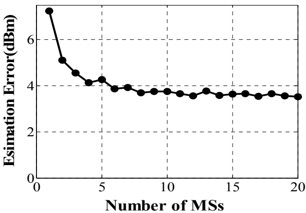
Fig. 6. Estimation error according as the increase of the number of participated MSs
