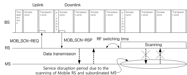
Fig. 1. Example of service disruption of MS due to the scanning of MRS
