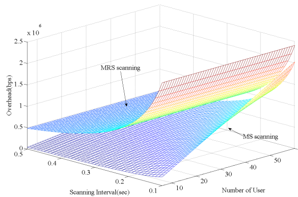
Fig. 8. Scanning overhead according to the scanning interval and the number of MS
