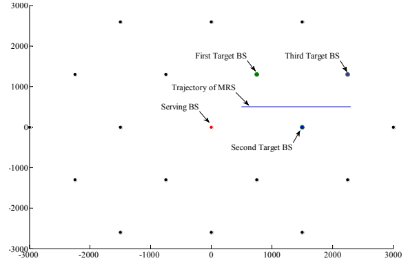
Fig. 3. BS deployment and the movement pattern of MRS (Unit: m)
