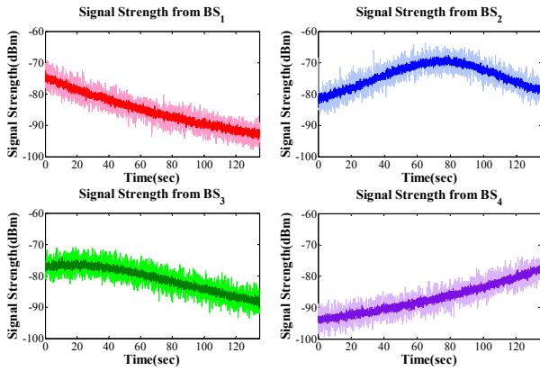
Fig. 5. Measured signal quality by MRS (light color) and estimated signal quality by proposed method (dark color)
