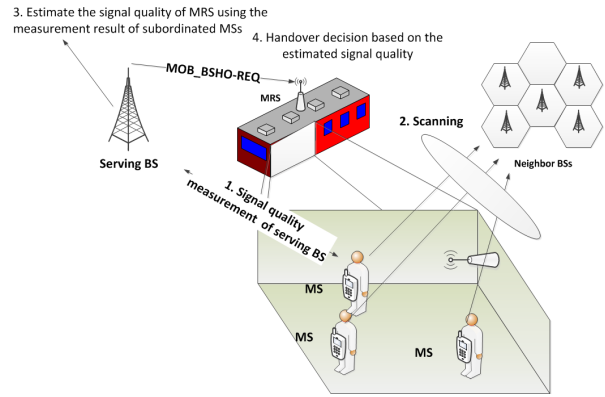
Fig. 2. Procedure of estimation-based scanning
