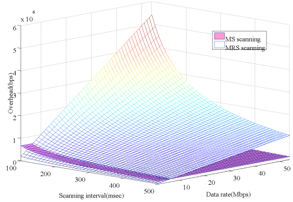
Fig. 7. Scanning overhead according to the scanning interval and data rate
