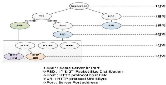
Fig. 3. Flow Grouping Diagram
