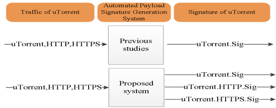
Fig. 1. Conceptual diagram of the automatic signature generation of multi-protocol-based application
