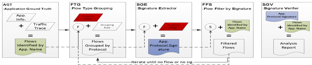
Fig. 2. Automated Payload Signature Generation Framework Structure
