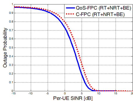
Fig. 9. Users outage probability under mixed flows using the C-FPC & the proposed QoS-FPC.
