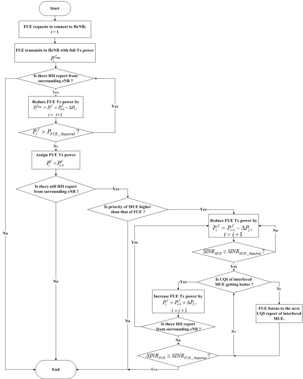
Fig. 3. Proposed UL power control scheme based on QoS priority.
