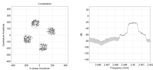
(a) Constellation of signal after RF cancellation (b) Spectrum of signal after RF cancellation
