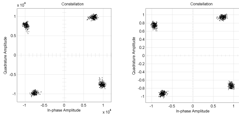
(a) Constellation of self-interference signal (b) Constellation of desired signal
